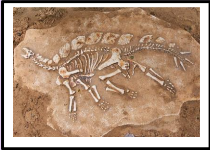
dinosaur fossil
